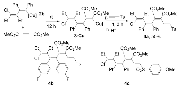
Scheme 5. Synthesis of Linear Tetraenes with Four Different Alkynes
